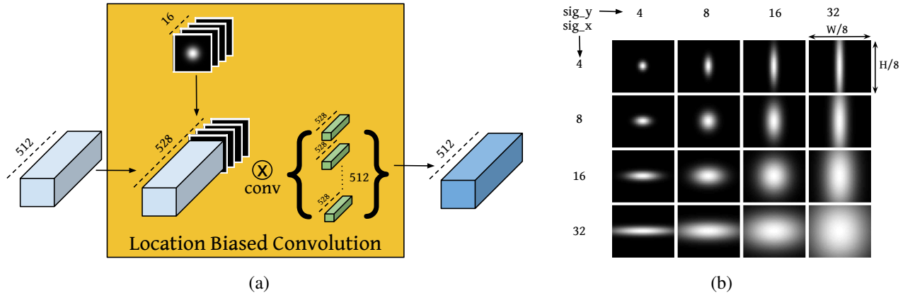
Fig. 5. (a). Location Biased Convolution Filter for learning location dependent patterns in data (e.g., centre-bias present in the eye-fixations). The usual bias term associated with convolutional layers and the ReLU activation are assumed to be present and are not shown explicitly in the above diagram. (b). Gaussian blobs with different horizontal and vertical variances concatenated to the input blob of LBC layers to make the layer’s response location specific.
