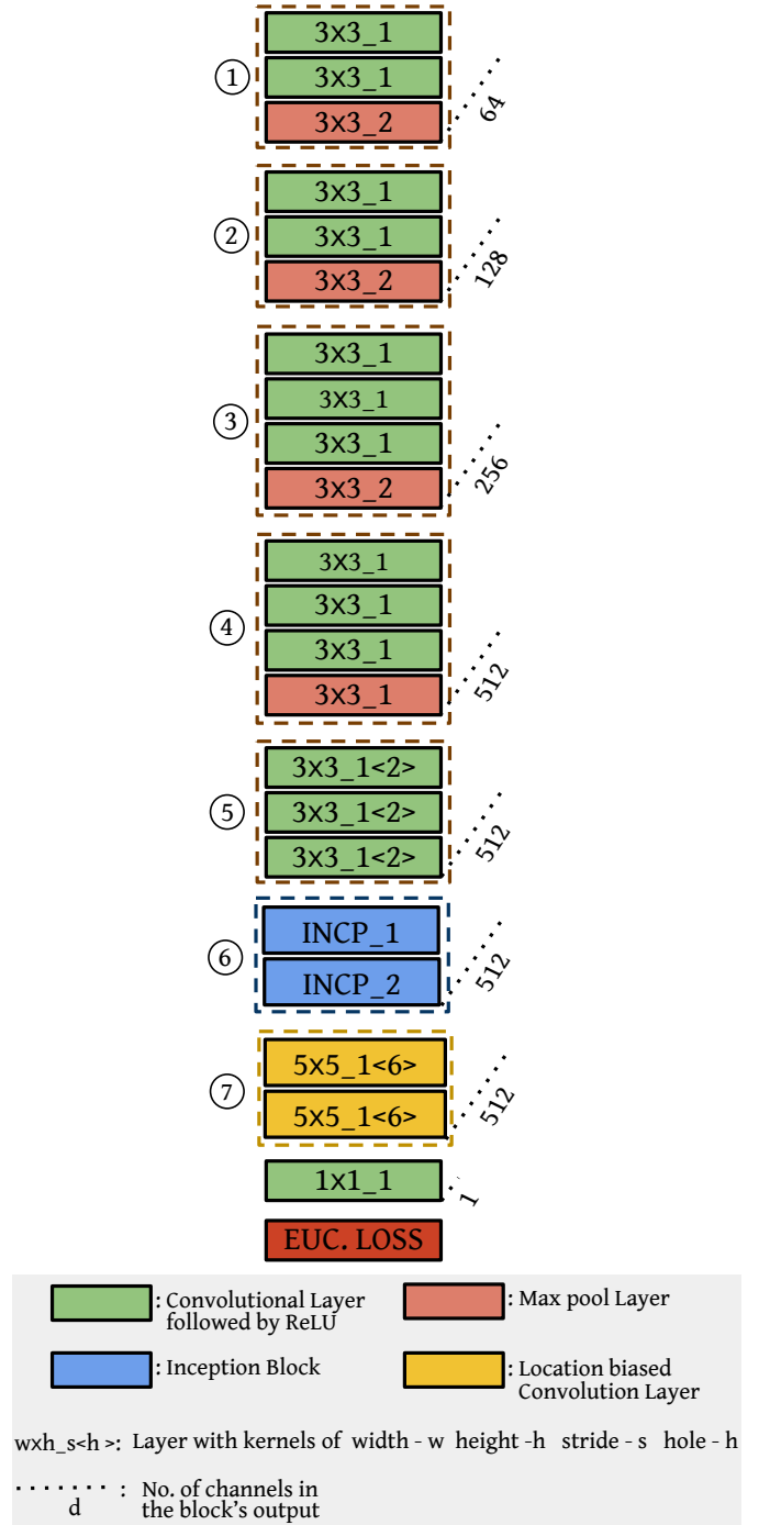
Fig. 2. Architecture of the proposed DeepFix model
