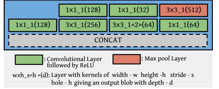
Fig. 4. Constituent layers of the Inception module used in DeepFix network
